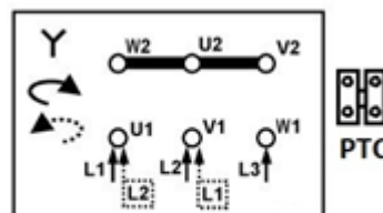
Star connection
